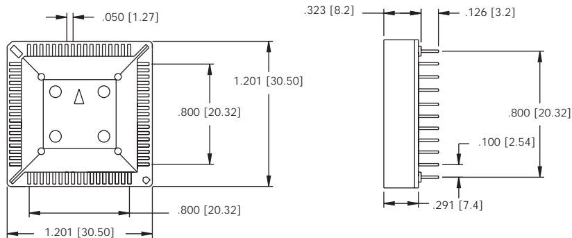
THIN WALL VERSION
