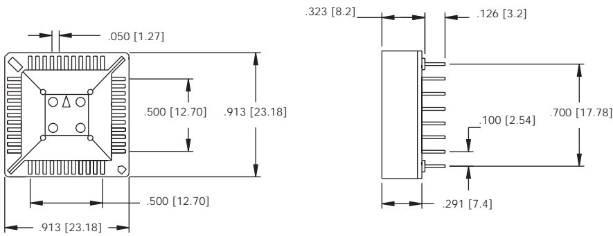
THIN WALL VERSION
