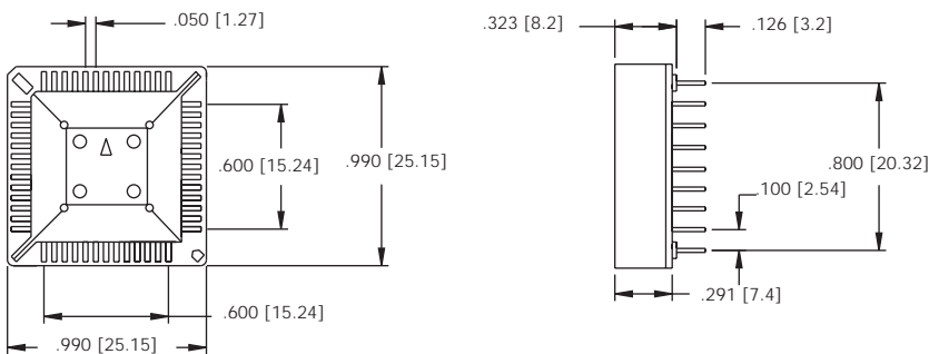
THIN WALL VERSION
