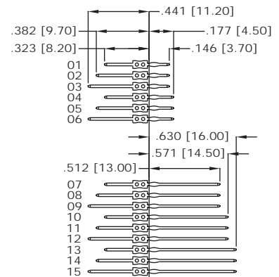
CONTACT DIMENSIONS
