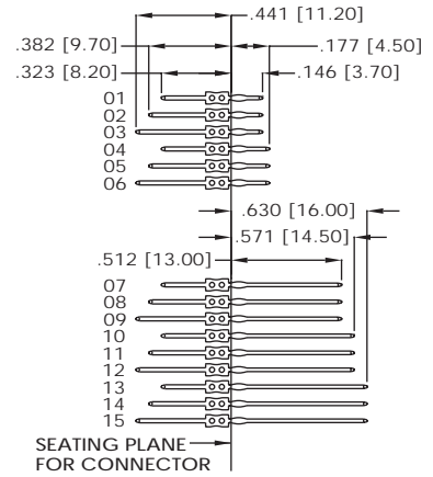
CONTACT DIMENSIONS
