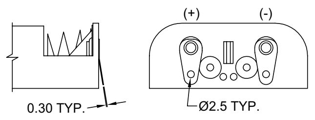
PDSN-14C SOLDER LUGS
