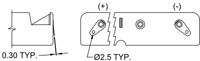
PDSN-14-2C SOLDER LUGS
