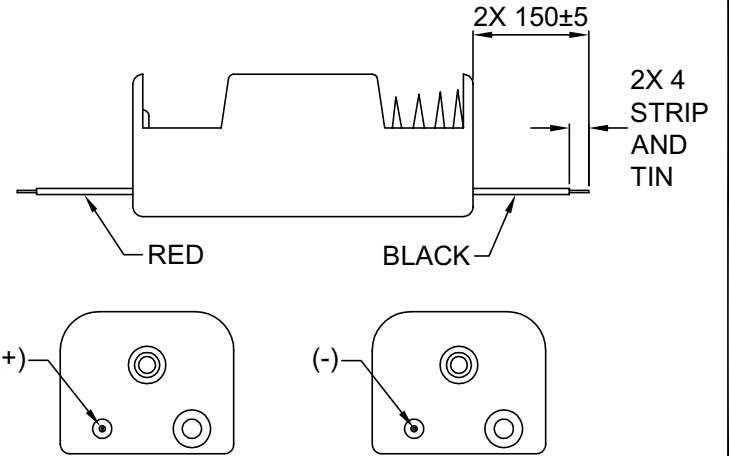
PDSN-11-1A WIRE LEADS
