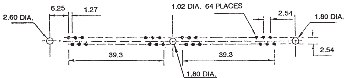
PCB LAYOUT
