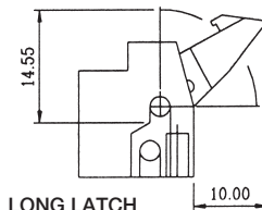
LONG LATCH FOR SOCKETS WITH STRAIN RELIEF
