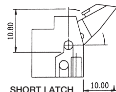
SHORT LATCH FOR SOCKETS WITHOUT STRAIN RELIEF
