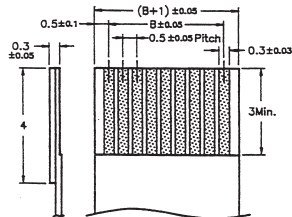
APPLICABLE FPC
