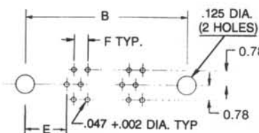
PCB LAYOUT 15 POSITIONS
