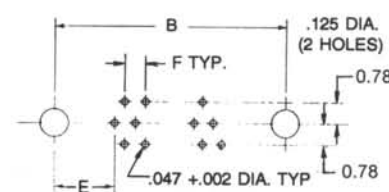
PCB LAYOUT 26, 44, 62 POSITIONS
