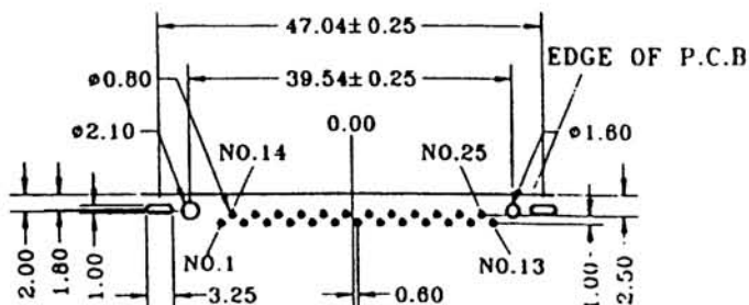
PCB LAYOUT
