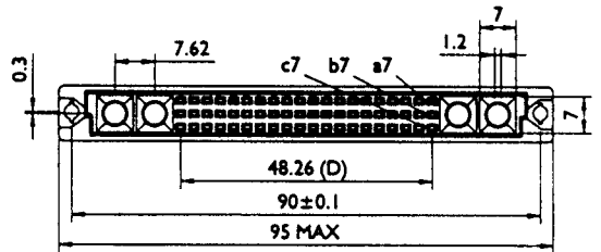
60 SIGNAL CONTACT LAYOUT
