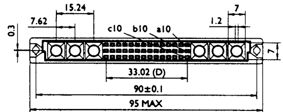
42 SIGNAL CONTACT LAYOUT
