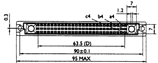
78 SIGNAL CONTACT LAYOUT
