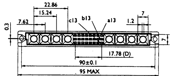
24 SIGNAL CONTACT LAYOUT
