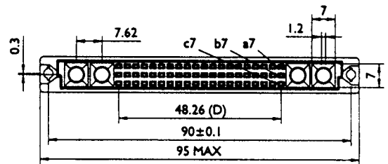
60 SIGNAL CONTACT LAYOUT
