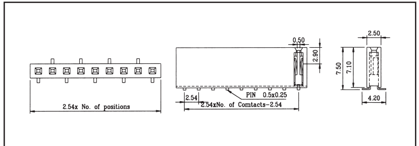
SINGLE ROW - DRAWING
