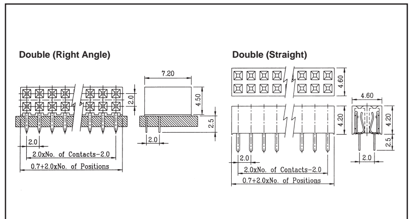
DOUBLE ROW - DRAWING
