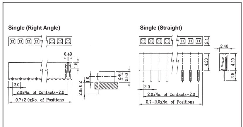
SINGLE ROW - DRAWING
