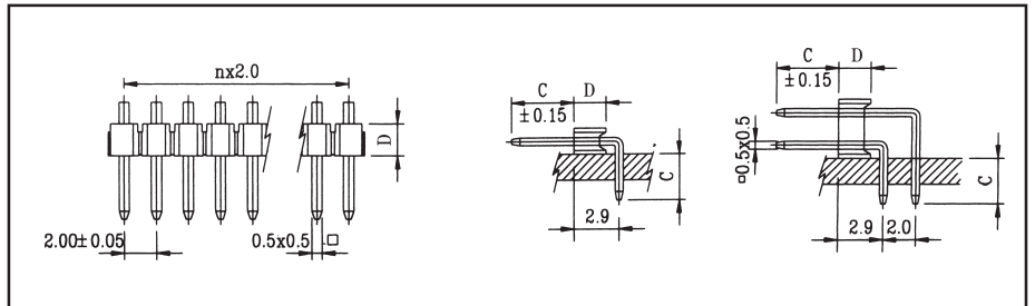
RIGHT ANGLE - DRAWING
