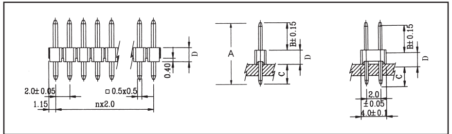
STRAIGHT - DRAWING
