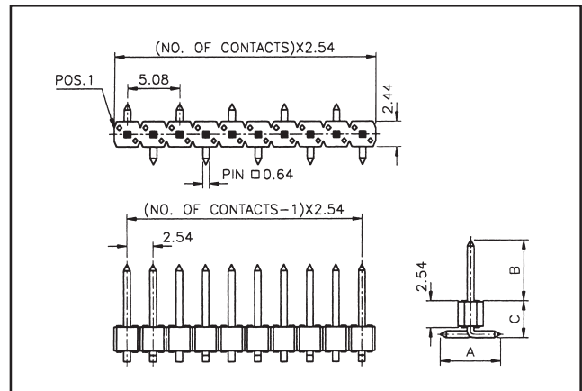
DRAWING
