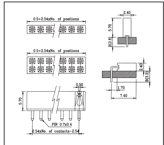
SINGLE ROW - DRAWING
