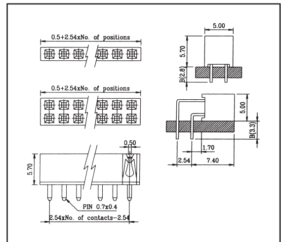
DUAL ROW - DRAWING
